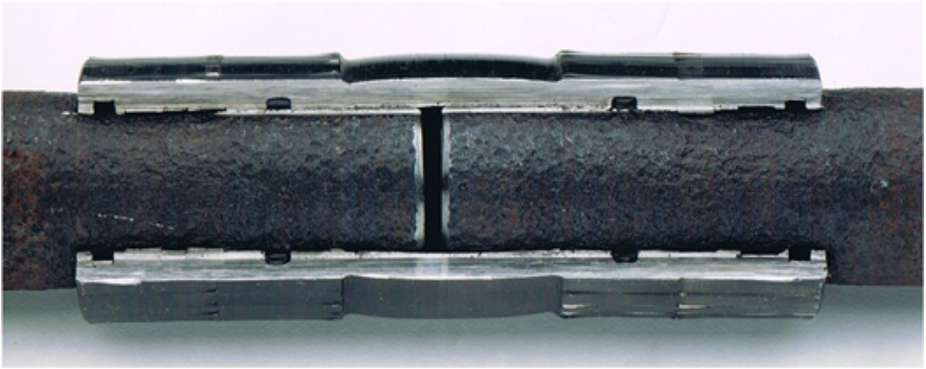
3/4" NPS Pipe-pitted due to years of exposure, Performed 6000 PSI Hydrostatic Proof Test and 1000 PSI Nitrogen Leak Test- No LEAKAGE DETECTED
